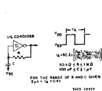
Fig. 18 - Astable multivibrator.
