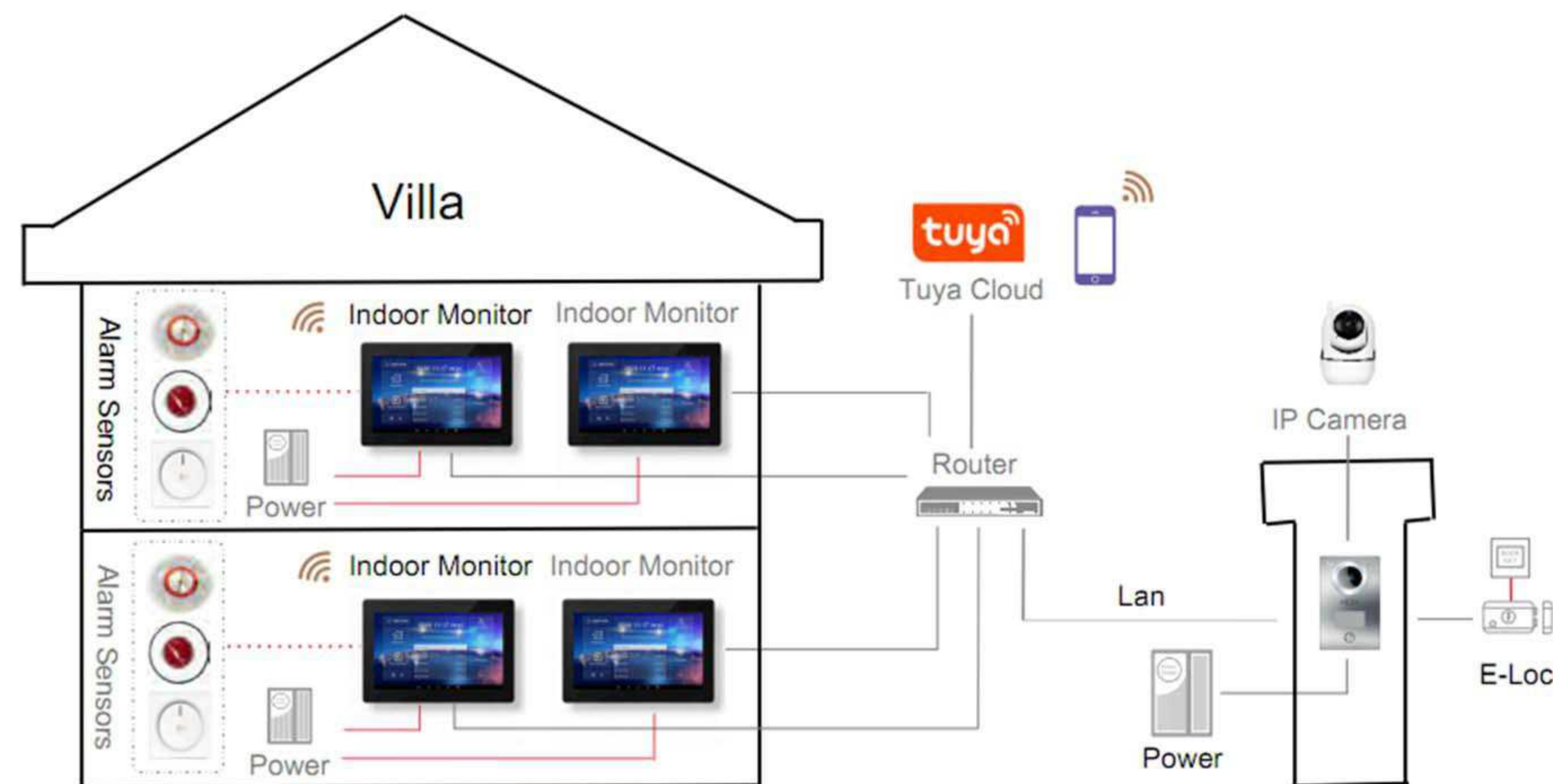
TC-5000MH-20H + TC-3000DA-X2
